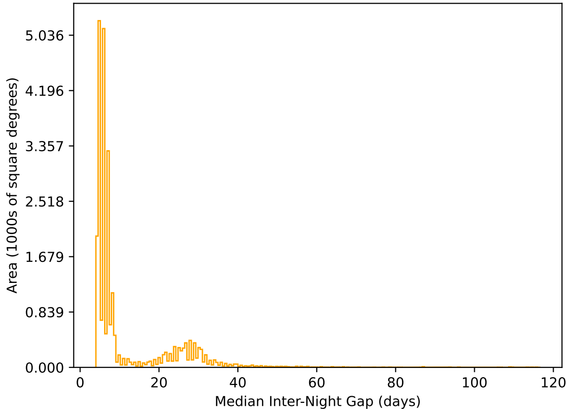
ddf_acor_sf10_lsf40_lsr10_v3.4_10yrs All sky r band: Median Inter-Night Gap
