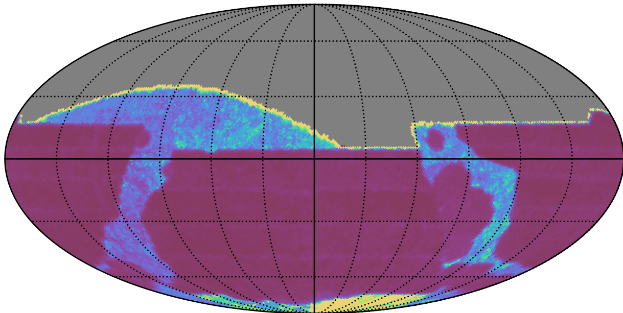
ddf_acor_sf10_lsf40_lsr10_v3.4_10yrs All sky i band: Median Inter-Night Gap
