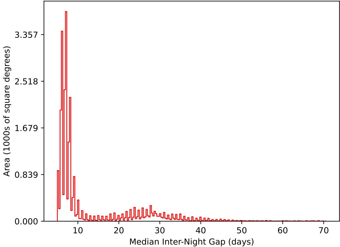
ddf_acor_sf10_lsf40_lsr10_v3.4_10yrs All sky i band: Median Inter-Night Gap
