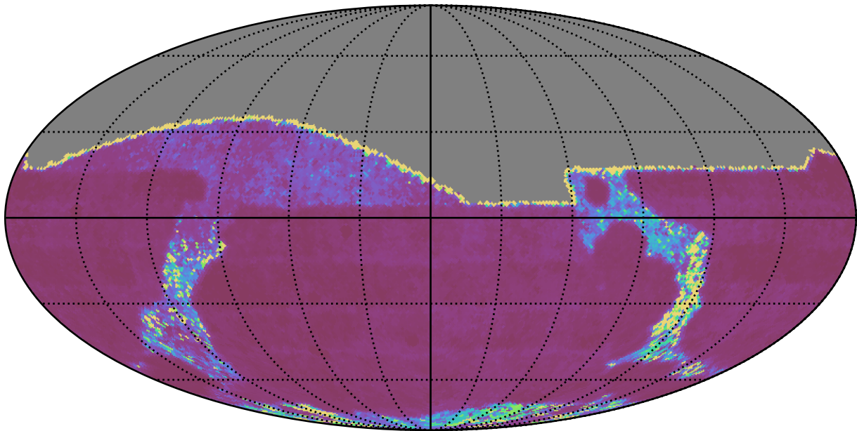
ddf_acor_sf10_lsf40_lsr10_v3.4_10yrs All sky g band: Median Inter-Night Gap
