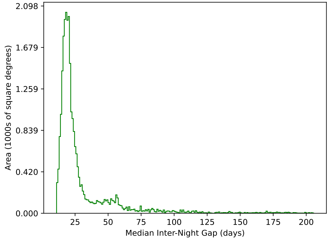
ddf_acor_sf10_lsf40_lsr10_v3.4_10yrs All sky g band: Median Inter-Night Gap
