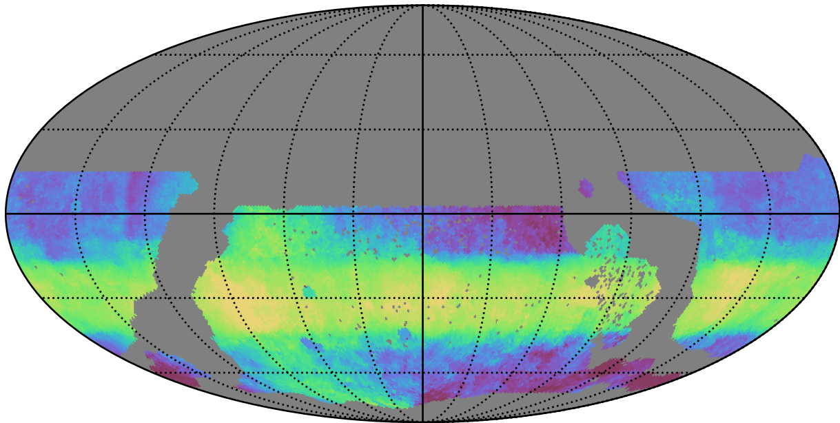
ddf_acor_sf10_lsf40_lsr10_v3.4_10yrs WFD z band: Median HA
