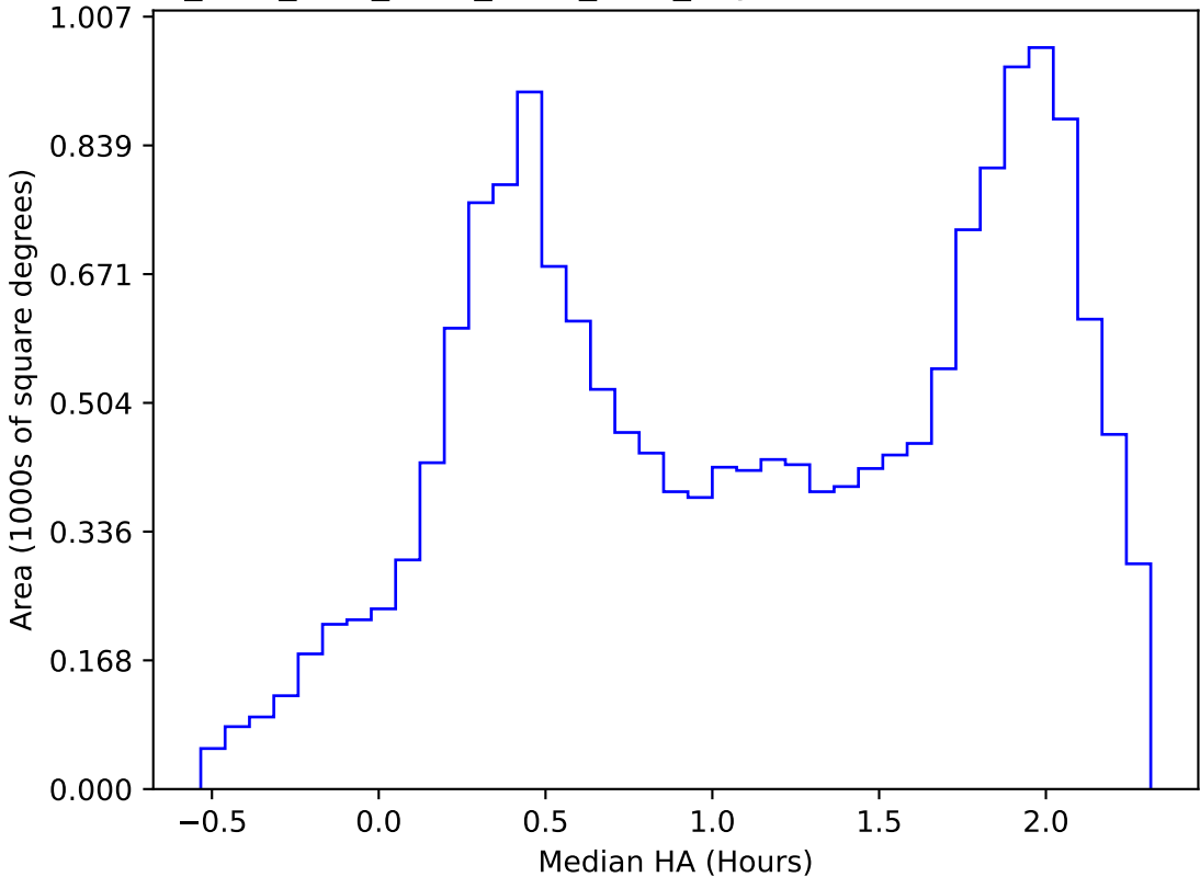
ddf_acor_sf10_lsf40_lsr10_v3.4_10yrs WFD z band: Median HA
