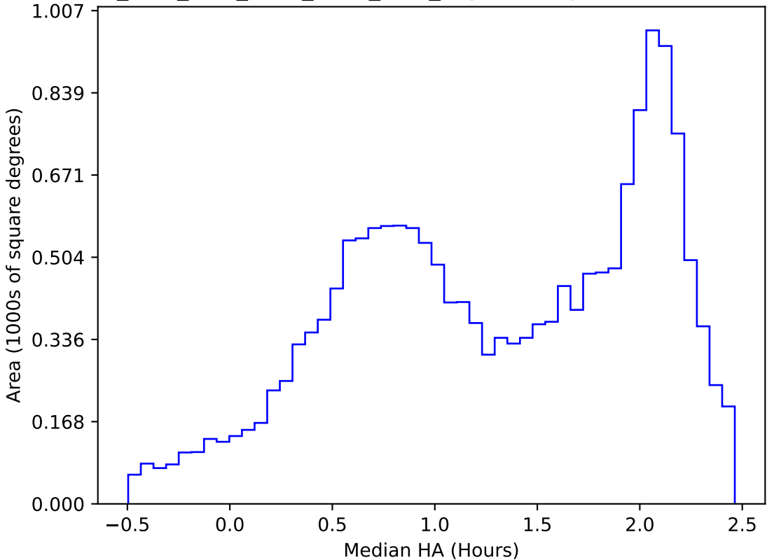
ddf_acor_sf10_lsf40_lsr10_v3.4_10yrs WFD y band: Median HA
