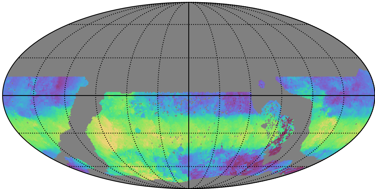
ddf_acor_sf10_lsf40_lsr10_v3.4_10yrs WFD u band: Median HA
