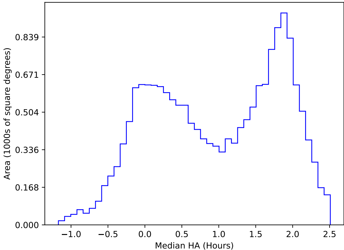
ddf_acor_sf10_lsf40_lsr10_v3.4_10yrs WFD u band: Median HA
