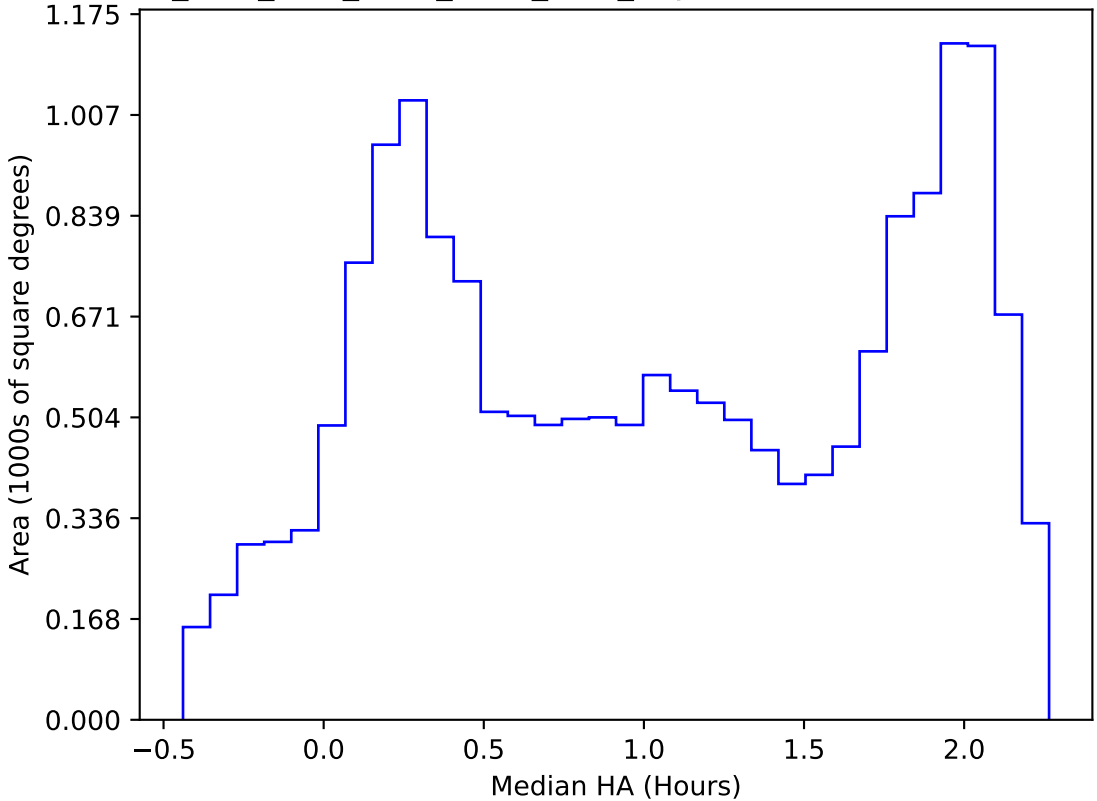
ddf_acor_sf10_lsf40_lsr10_v3.4_10yrs WFD i band: Median HA
