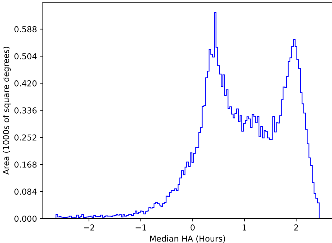
ddf_acor_sf10_lsf40_lsr10_v3.4_10yrs All sky z band: Median HA
