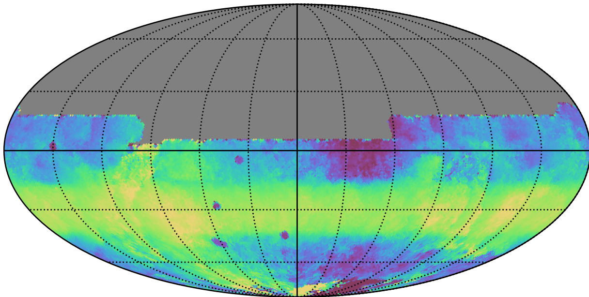
ddf_acor_sf10_lsf40_lsr10_v3.4_10yrs All sky y band: Median HA
