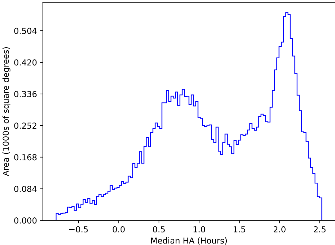
ddf_acor_sf10_lsf40_lsr10_v3.4_10yrs All sky y band: Median HA
