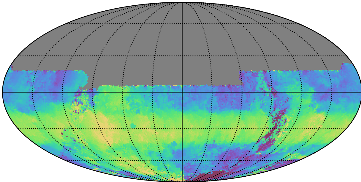
ddf_acor_sf10_lsf40_lsr10_v3.4_10yrs All sky u band: Median HA
