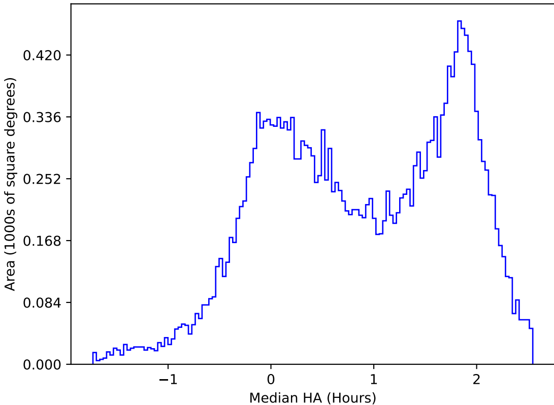
ddf_acor_sf10_lsf40_lsr10_v3.4_10yrs All sky u band: Median HA
