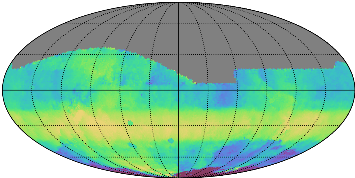
ddf_acor_sf10_lsf40_lsr10_v3.4_10yrs All sky r band: Median HA
