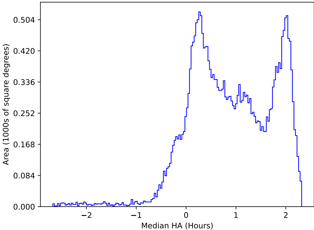
ddf_acor_sf10_lsf40_lsr10_v3.4_10yrs All sky i band: Median HA
