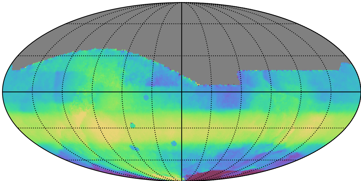
ddf_acor_sf10_lsf40_lsr10_v3.4_10yrs All sky all bands: Median HA
