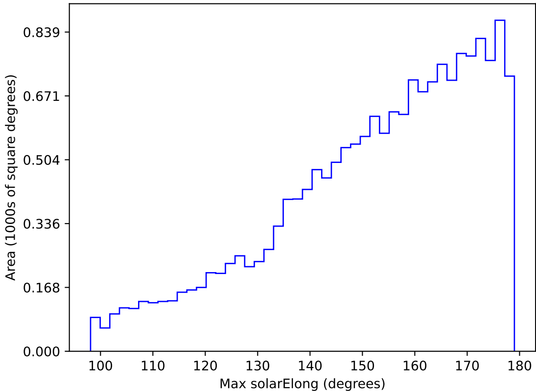
ddf_acor_sf10_lsf40_lsr10_v3.4_10yrs WFD u band: Max solarElong
