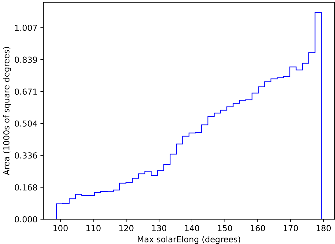
ddf_acor_sf10_lsf40_lsr10_v3.4_10yrs WFD r band: Max solarElong
