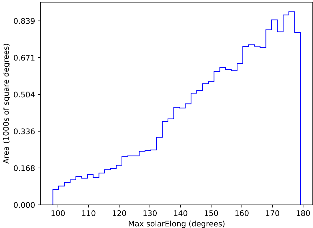
ddf_acor_sf10_lsf40_lsr10_v3.4_10yrs WFD g band: Max solarElong
