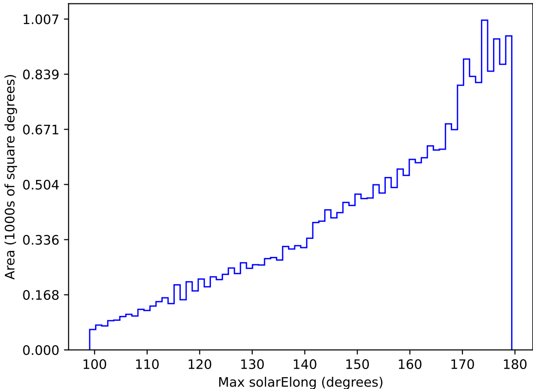
ddf_acor_sf10_lsf40_lsr10_v3.4_10yrs All sky z band: Max solarElong
