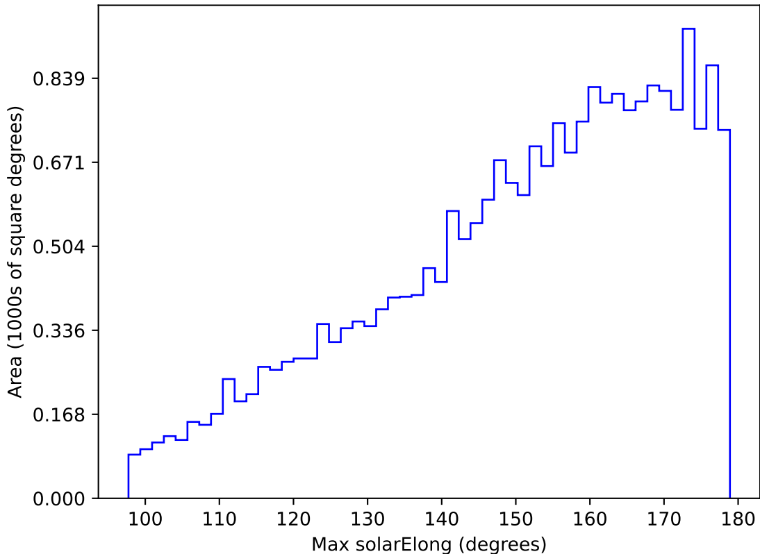
ddf_acor_sf10_lsf40_lsr10_v3.4_10yrs All sky u band: Max solarElong
