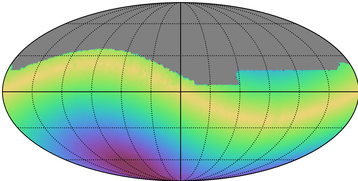
ddf_acor_sf10_lsf40_lsr10_v3.4_10yrs All sky r band: Max solarElong
