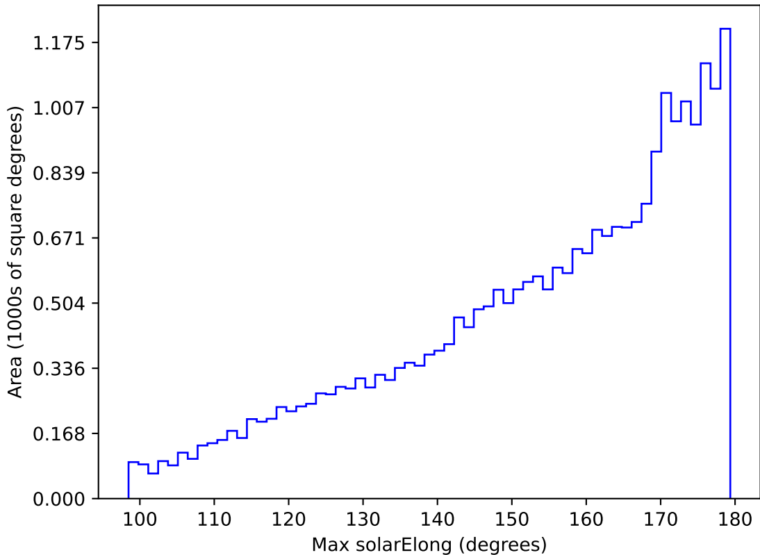
ddf_acor_sf10_lsf40_lsr10_v3.4_10yrs All sky r band: Max solarElong
