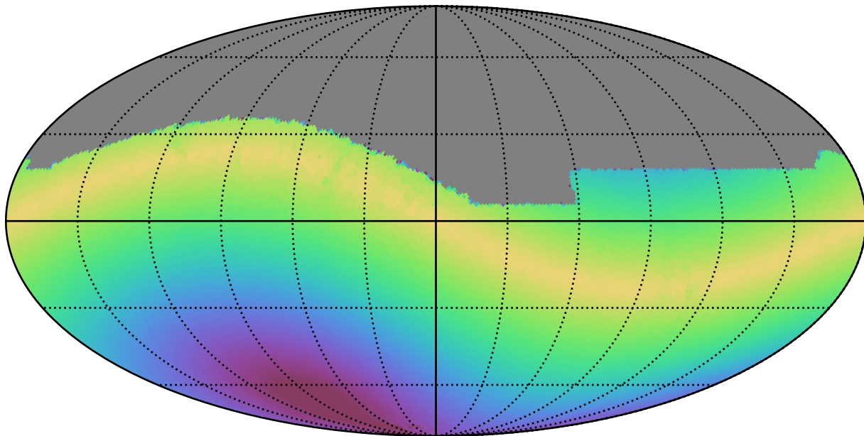
ddf_acor_sf10_lsf40_lsr10_v3.4_10yrs All sky i band: Max solarElong
