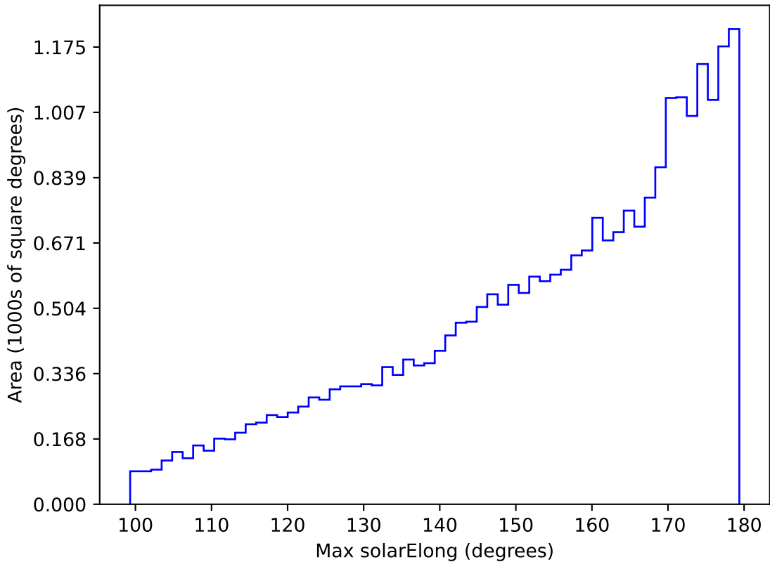
ddf_acor_sf10_lsf40_lsr10_v3.4_10yrs All sky i band: Max solarElong
