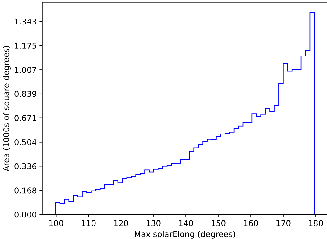
ddf_acor_sf10_lsf40_lsr10_v3.4_10yrs All sky all bands: Max solarElong
