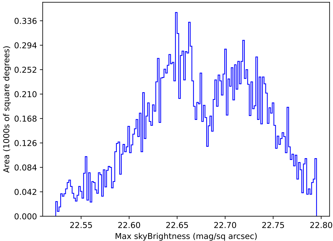
ddf_acor_sf10_lsf40_lsr10_v3.4_10yrs Yr 1 u band: Max skyBrightness
