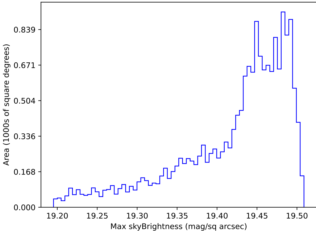
ddf_acor_sf10_lsf40_lsr10_v3.4_10yrs WFD z band: Max skyBrightness
