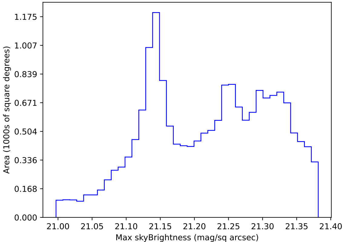
ddf_acor_sf10_lsf40_lsr10_v3.4_10yrs WFD r band: Max skyBrightness
