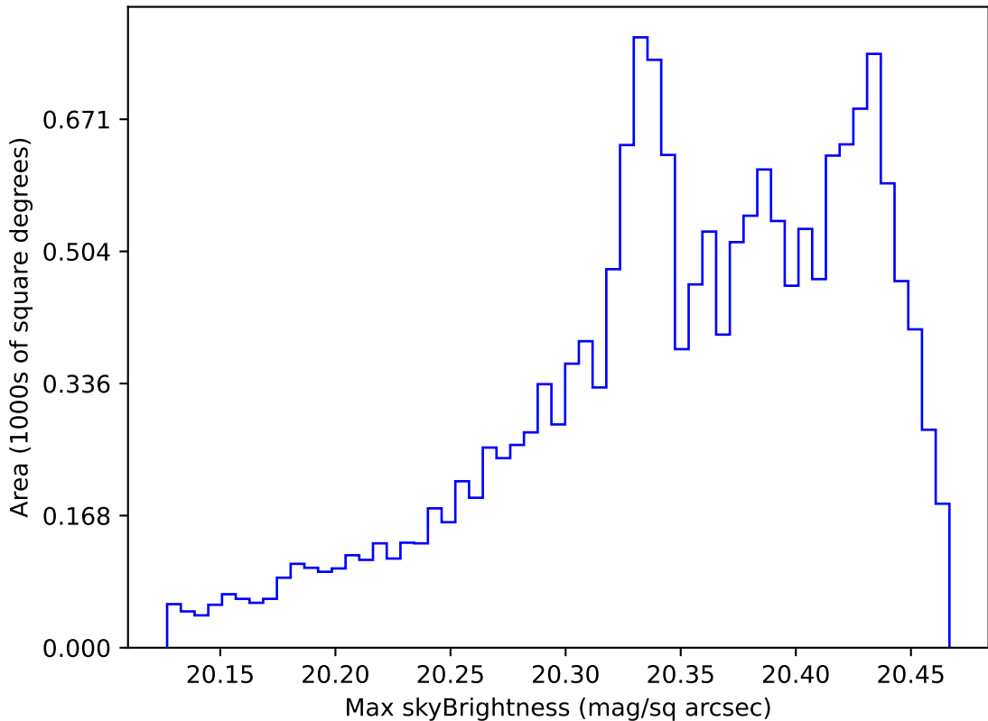
ddf_acor_sf10_lsf40_lsr10_v3.4_10yrs WFD i band: Max skyBrightness
