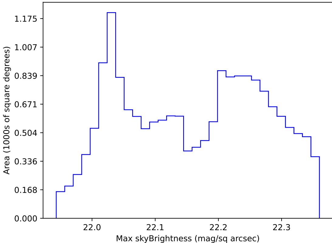
ddf_acor_sf10_lsf40_lsr10_v3.4_10yrs WFD g band: Max skyBrightness
