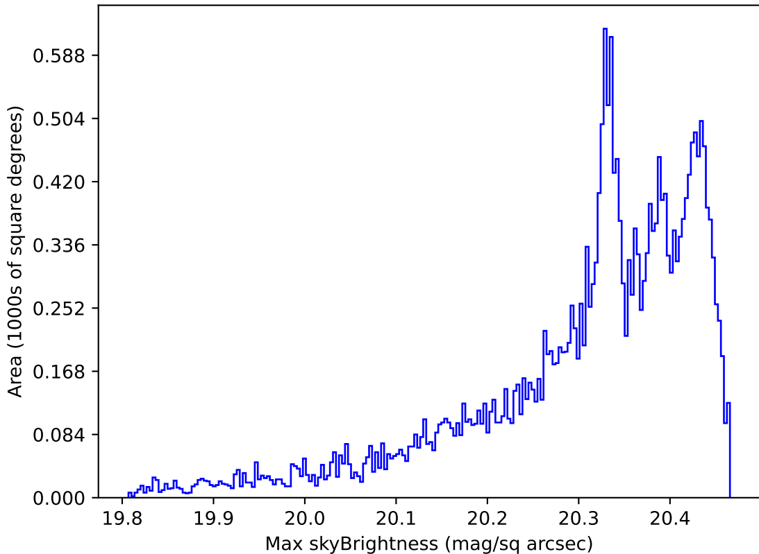
ddf_acor_sf10_lsf40_lsr10_v3.4_10yrs All sky i band: Max skyBrightness
