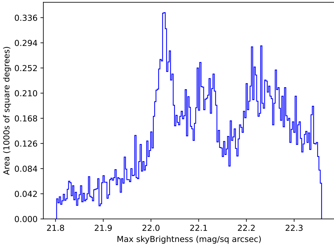
ddf_acor_sf10_lsf40_lsr10_v3.4_10yrs All sky g band: Max skyBrightness
