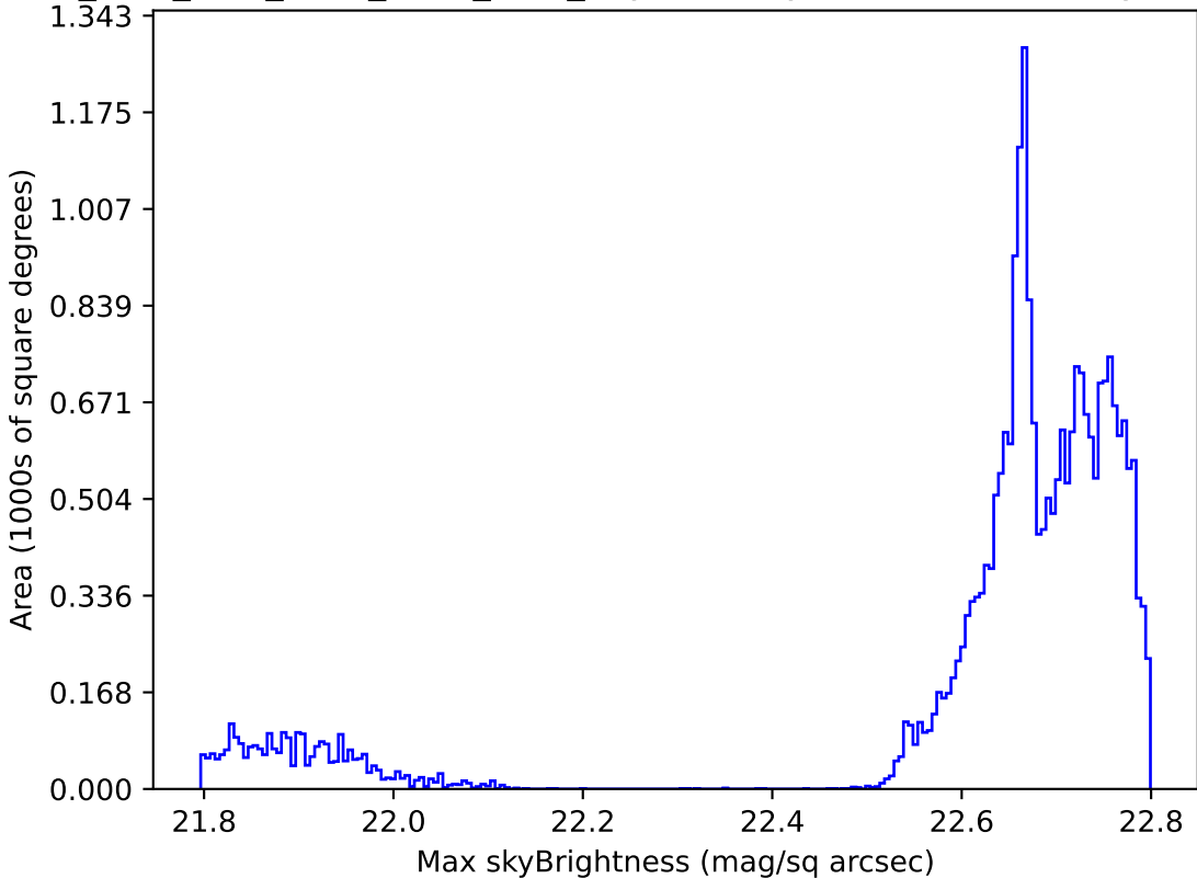
ddf_acor_sf10_lsf40_lsr10_v3.4_10yrs All sky all bands: Max skyBrightness
