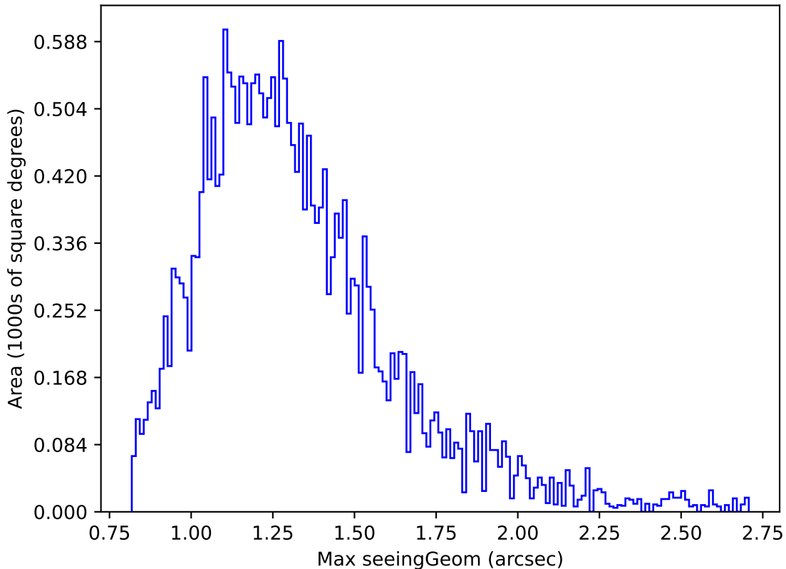
ddf_acor_sf10_lsf40_lsr10_v3.4_10yrs Yr 1 g band: Max seeingGeom
