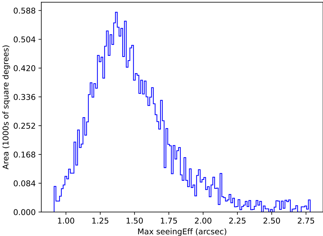
ddf_acor_sf10_lsf40_lsr10_v3.4_10yrs Yr 1 y band: Max seeingEff
