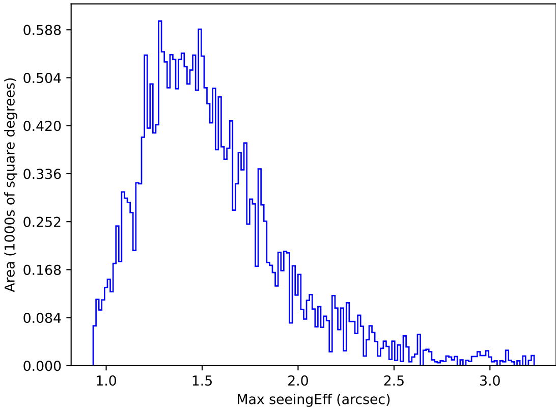
ddf_acor_sf10_lsf40_lsr10_v3.4_10yrs Yr 1 g band: Max seeingEff
