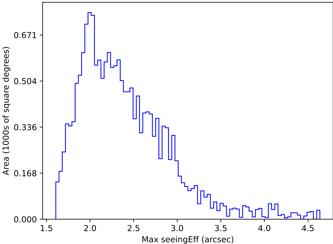
ddf_acor_sf10_lsf40_lsr10_v3.4_10yrs WFD y band: Max seeingEff
