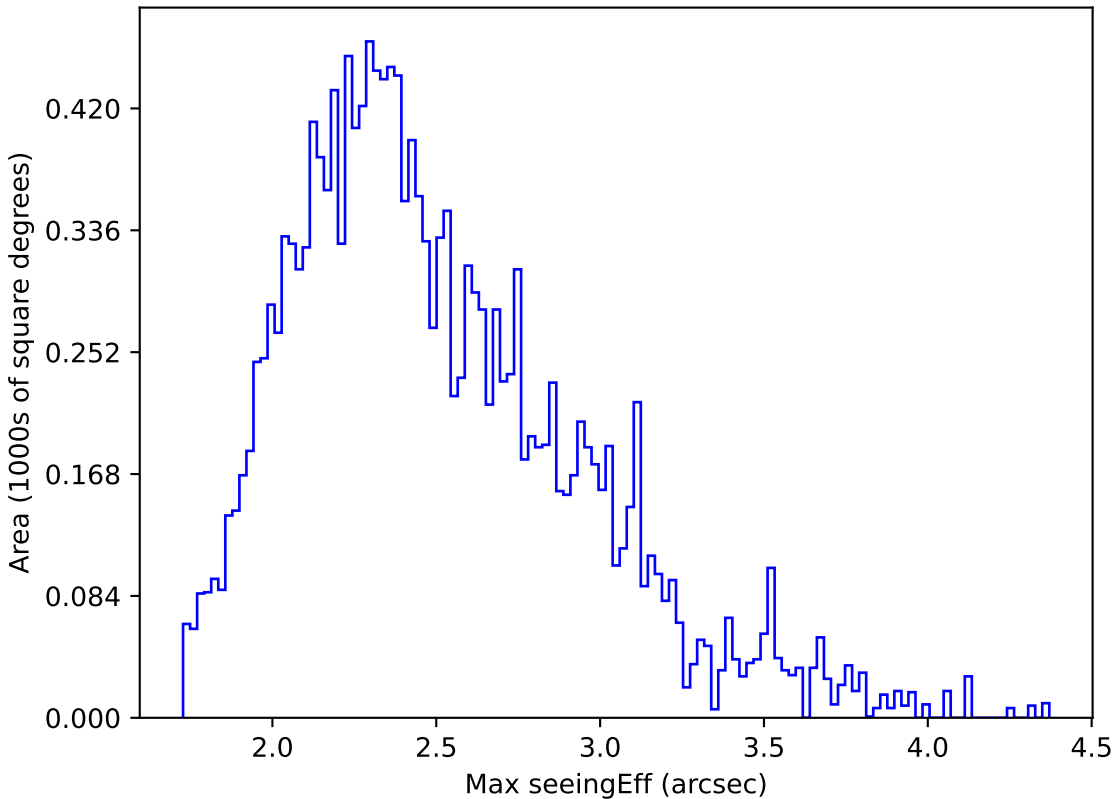
ddf_acor_sf10_lsf40_lsr10_v3.4_10yrs WFD u band: Max seeingEff
