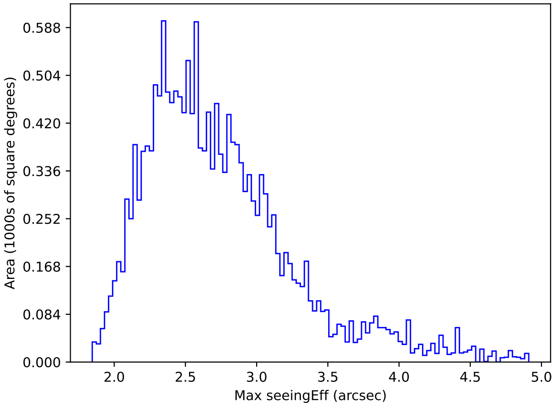
ddf_acor_sf10_lsf40_lsr10_v3.4_10yrs WFD r band: Max seeingEff
