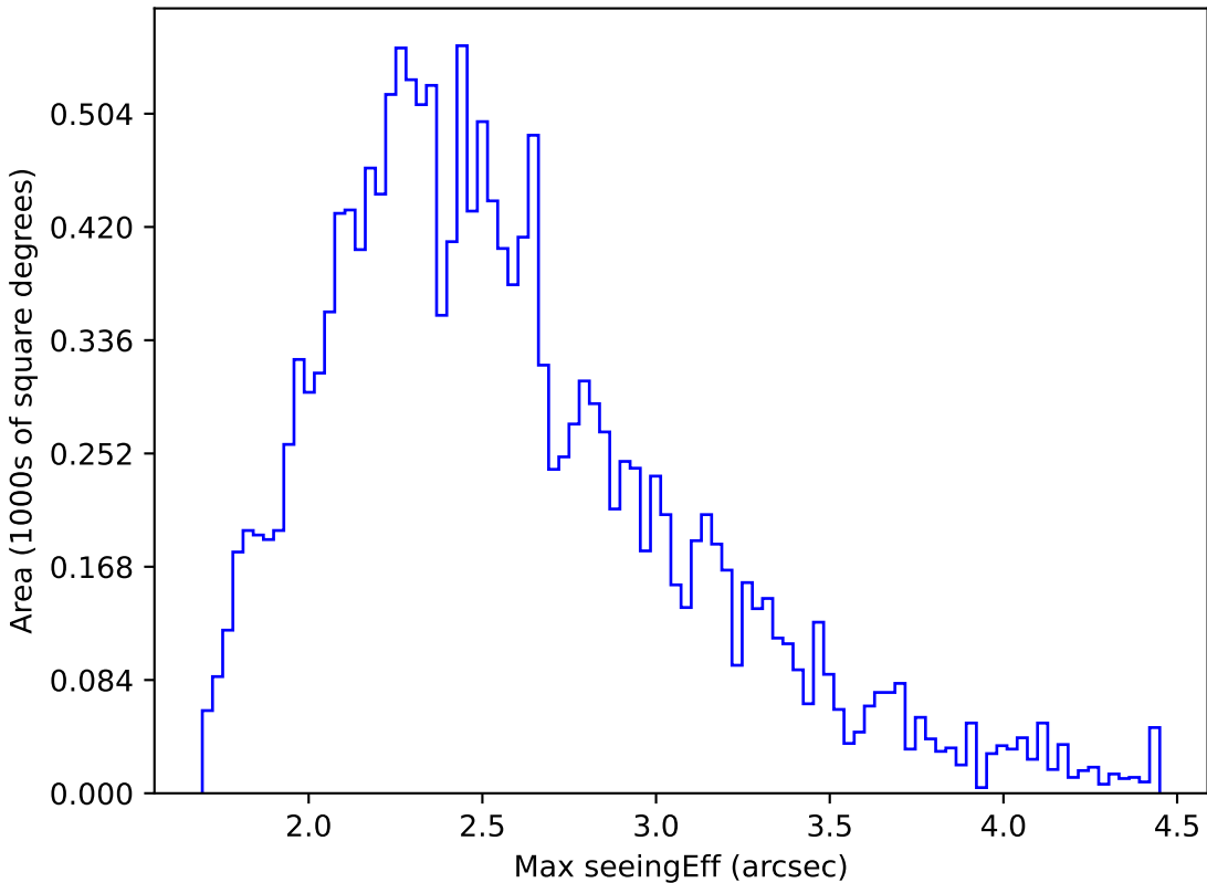
ddf_acor_sf10_lsf40_lsr10_v3.4_10yrs WFD g band: Max seeingEff
