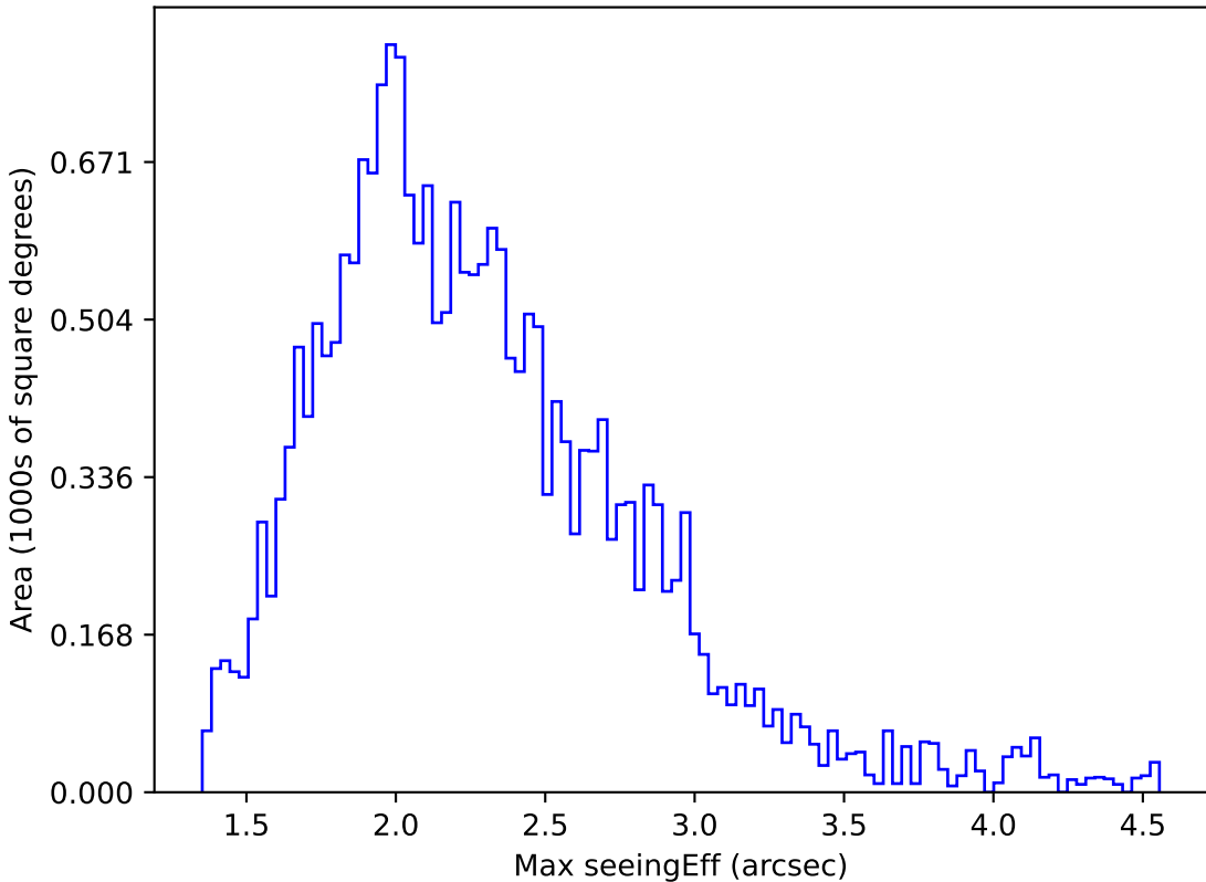
ddf_acor_sf10_ls40_lsr10_v3.4_10yrs All sky y band: Max seeingEff
