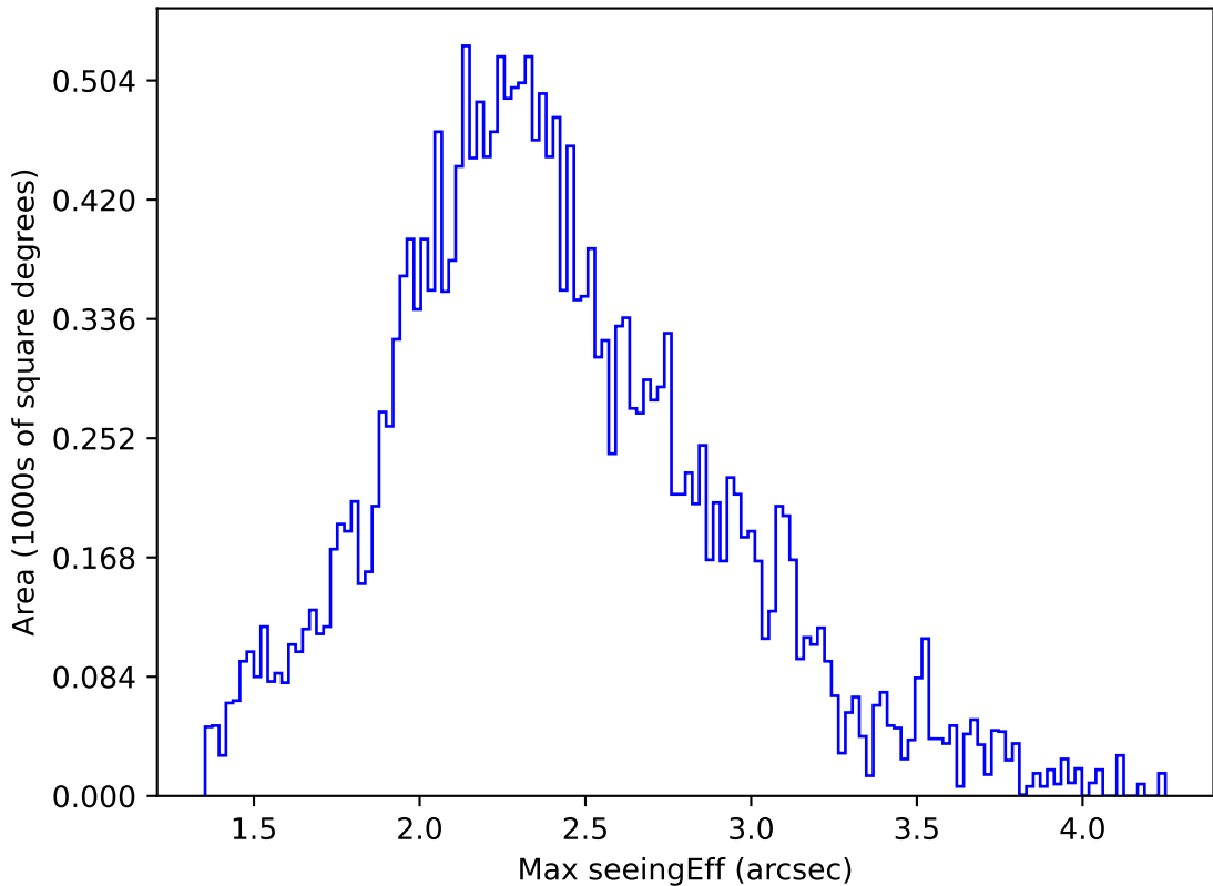
ddf_acor_sf10_ls40_lsr10_v3.4_10yrs All sky u band: Max seeingEff
