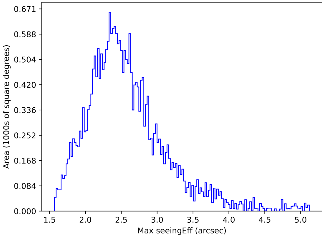
ddf_acor_sf10_lsf40_lsr10_v3.4_10yrs All sky i band: Max seeingEff
