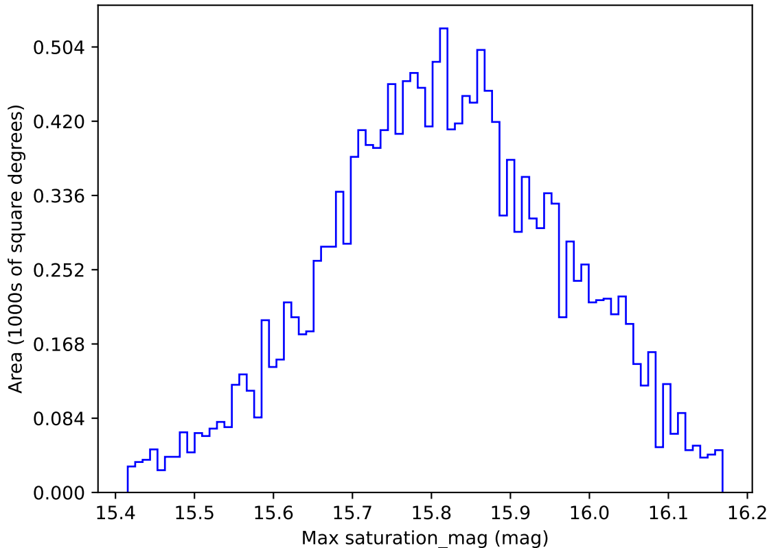
ddf_acor_sf10_lsf40_lsr10_v3.4_10yrs WFD all bands: Max saturation_mag
