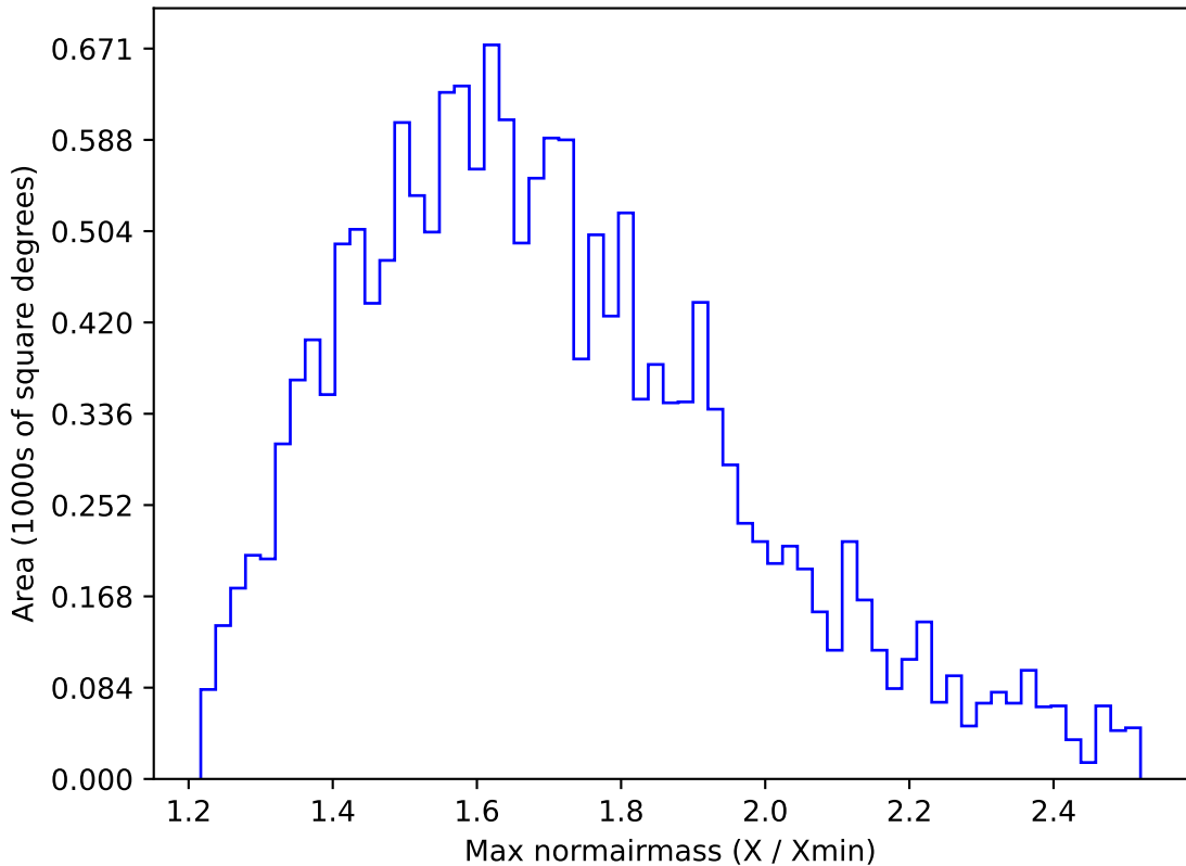
ddf_acor_sf10_lsf40_lsr10_v3.4_10yrs WFD u band: Max normairmass
