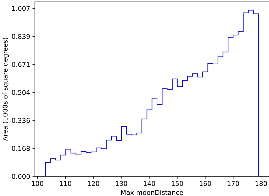
ddf_acor_sf10_ls40_lsr10_v3.4_10yrs WFD g band: Max moonDistance
